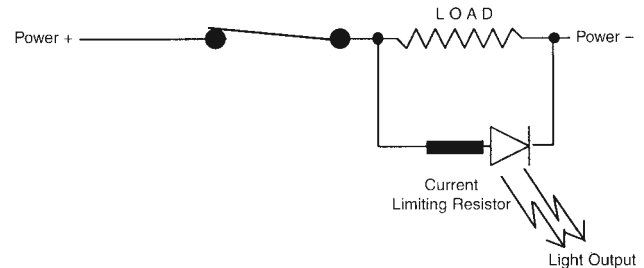
Figure 19. Wiring Diagram 4
