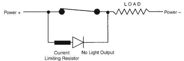
Figure 17. Wiring Diagram 2
