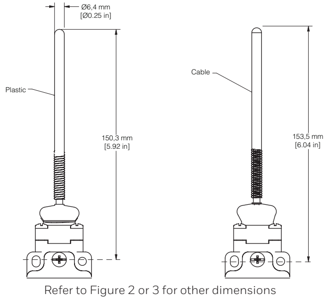
Figure 10. Plastic Rod and Flexible Cable
