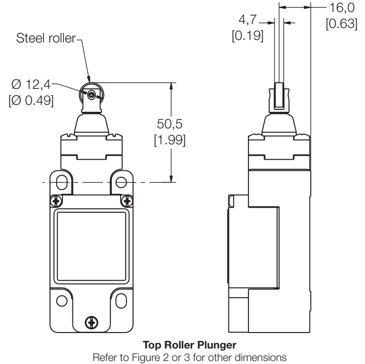
Figure 7. Roller Plunger Dimensions
