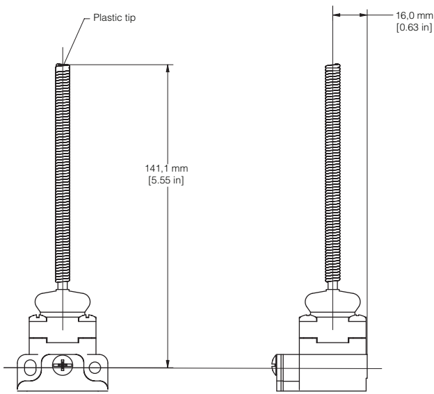
Figure 9. Coil Actuator
