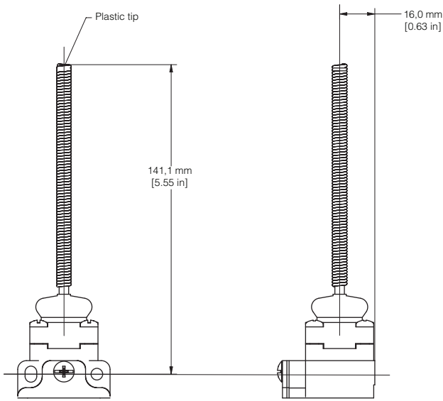
Figure 9. Coil Actuator
