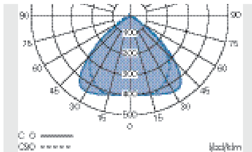
Polar curve eLLK/M 92 LED 400A/800A
