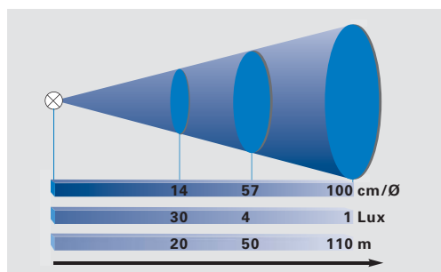
Range-diagram SEB 9 / 8
