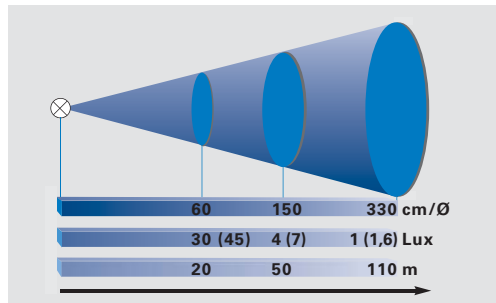
Range-diagram SEB 10
