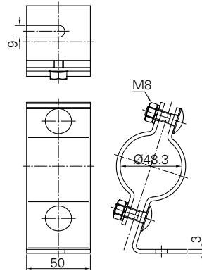
Pipe clamp LB 48 - FT
