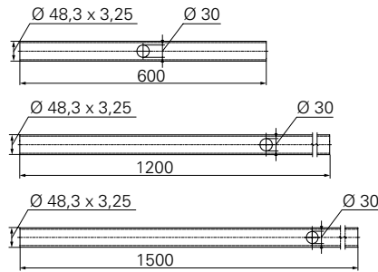
Light fitting support pipe with cable outlet
