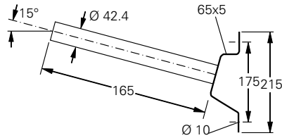
Wandarm W27
