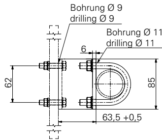
LMHW 48 - FT
