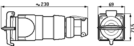
Coupler, GHG 513
