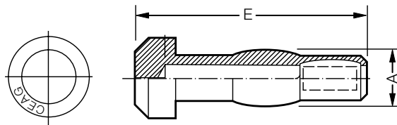
Blanking plug
