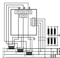
3-PHASE 4-WIRE (3P/4W) UNBALANCED
