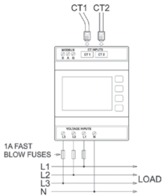
3 phase, 4-wire
