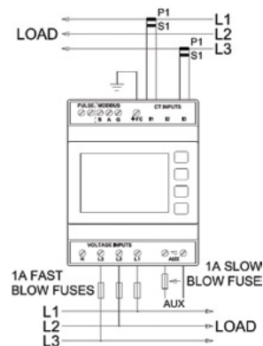
3-phase, 3-wire
