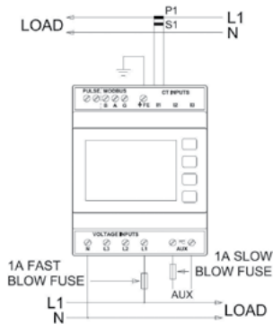
Single-phase, 2-wire
