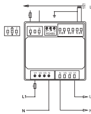
1-phase 2-wire
