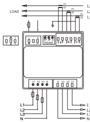
3-phase 4-wire
