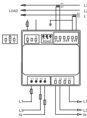
3-phase 3-wire
