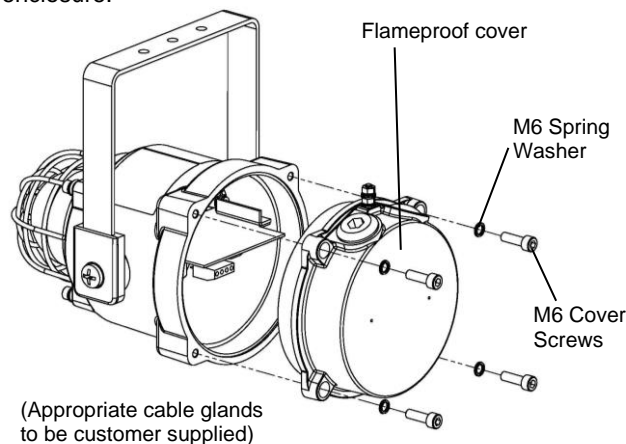
Fig. 2 Accessing the Explosion proof Enclosure.
