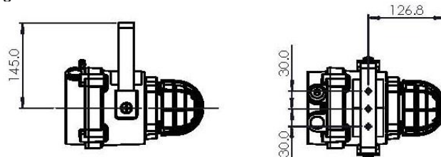
Fig 1. Fixing Location for Beacon
