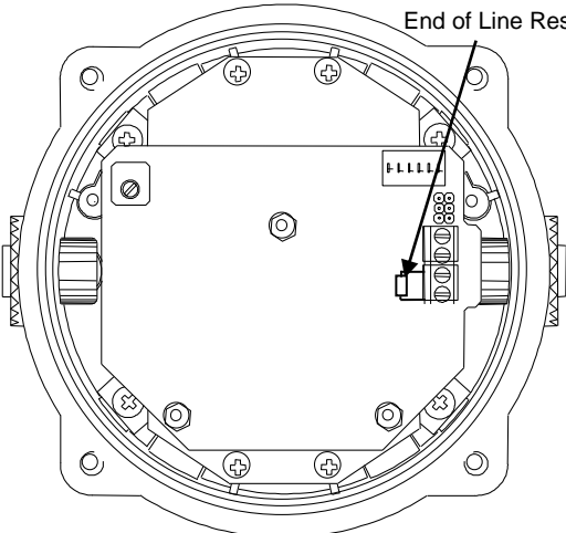
Fig. 8 End of Line Resistor Placement
