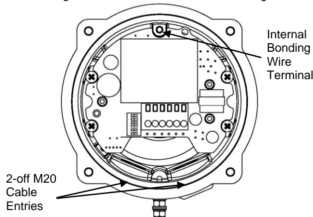
Fig. 3b Internal View of Cover
