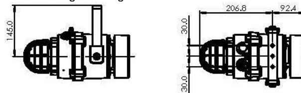
Fig. 1 Fixing Location for Combined Radial
