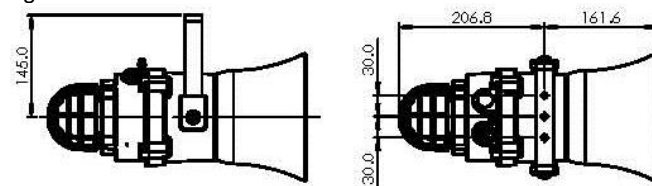
Fig. 1 Fixing Location for Combined Flare
