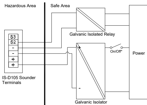
Fig 8 Multi stage alarm using galvanic isolated relays
