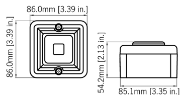
Multi-purpose Backbox
