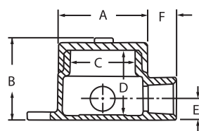
XTF Type With Mounting Flange
