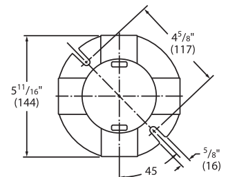
XTF Type With Mounting Flange
