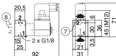
TYPE 04 Single subbase Zamak 35300047
