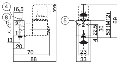
TYPE 04 Single subbase Zamak 35300047
