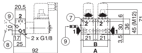
TYPE 05 Joinable subbase Zamak 35300048
