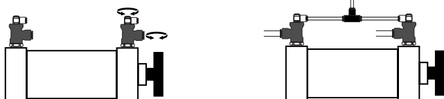
Cylinder in movement (pilot pressure applied)
