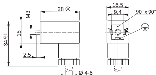
TYPE 03 Size 15, flying leads, without LED indicator EN 175301-803, industry standard form C (9,4 mm) IP65 (non-rotatable terminal holder)
