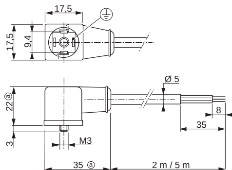
TYPE 04 Size 15, flying leads, with LED indicator EN 175301-803, industry standard form C (9,4 mm) IP65 (non-rotatable terminal holder)
