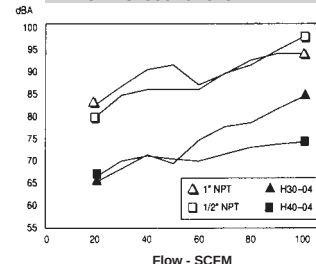
Air flow vs. sound level
