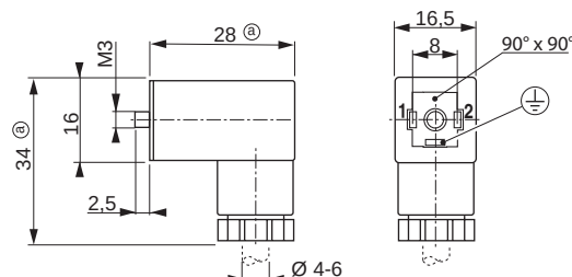
TYPE 02 Size 15, 8 mm EN 175301-803, form C IP65
