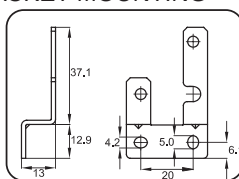
Bracket for vertical mounting
