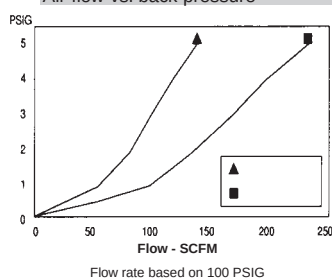
Air flow vs. back pressure
