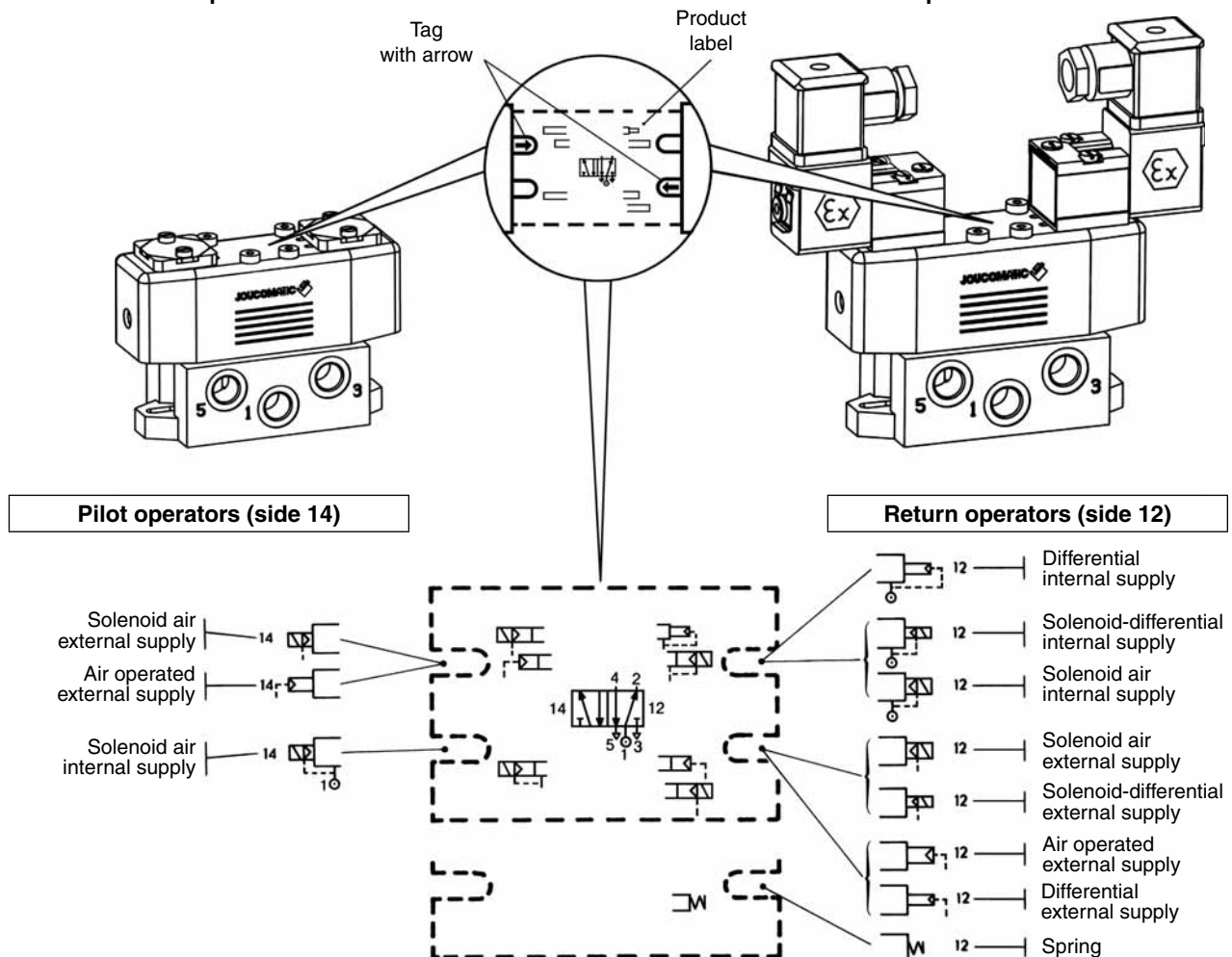
Air operated spool valve
