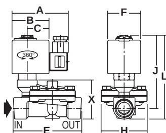
TYPE 03 Prefix "SC" Solenoid Epoxy moulded IEC 335 / ISO 4400 IP65
