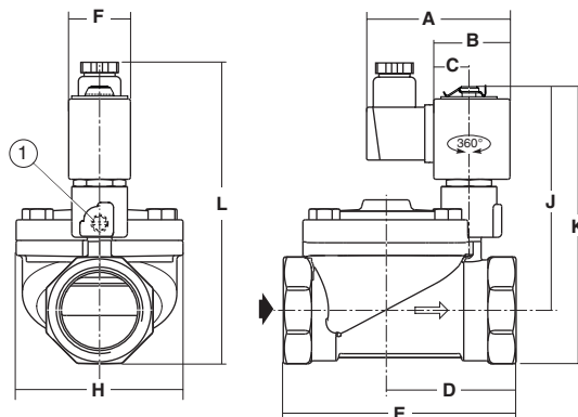
TYPE 03 Prefix "SC" Solenoid Black PPS moulded IEC 335 / ISO 4400 IP65
