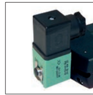
TYPE 02: Epoxy moulded SC: IEC 335 / ISO 4400
