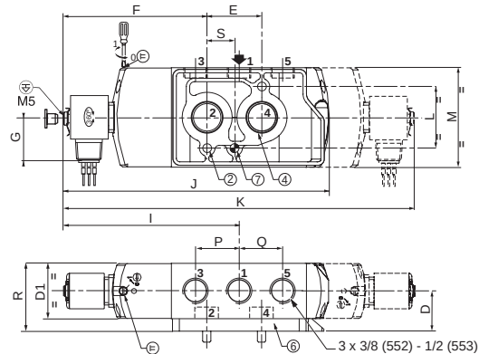
TYPE 10: Epoxy encapsulated JBEF: NEMA type 7, 9
