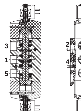
bistable (553 Series)
