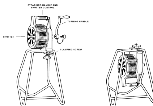
SIREN assembled for use Height: 84cm Width: 37cm Depth: 48cm
