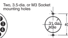
Mounting Holes
