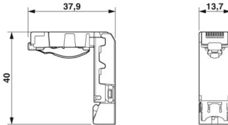
Dimensional drawing
