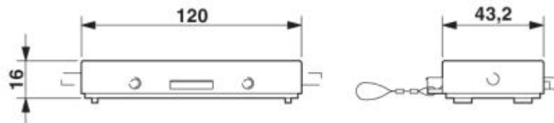
Dimensional drawing
