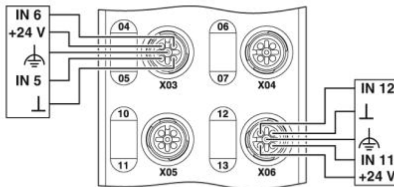
Connection diagram
