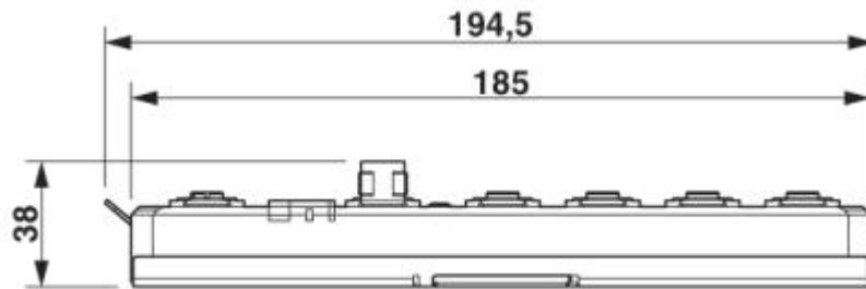
Dimensional drawing
