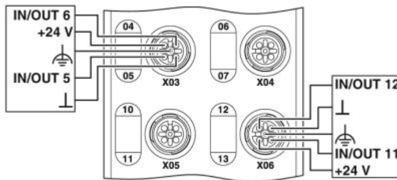
Connection diagram
