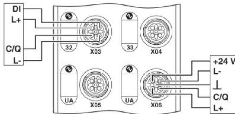
Connection diagram
