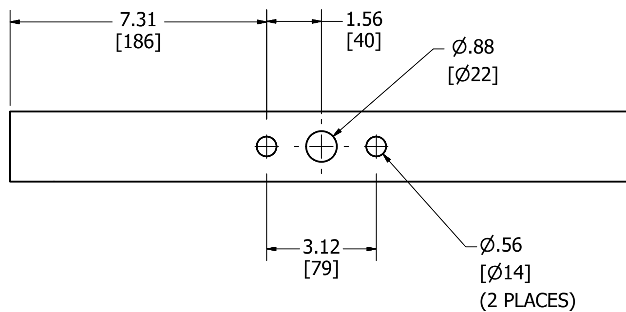
TRUNNION MOUNTING DETAIL
