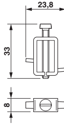
Dimensional drawing
