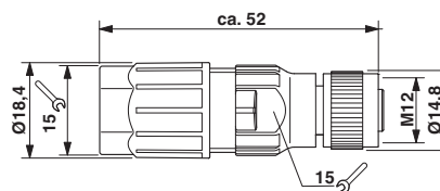
Dimensional drawing
