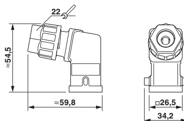
Dimensional drawing
