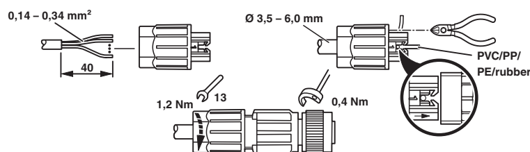
Functional drawing
