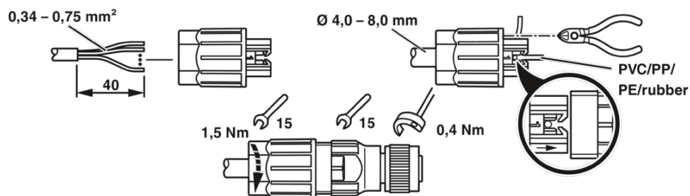
Functional drawing
