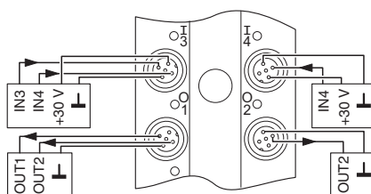
Connection diagram
