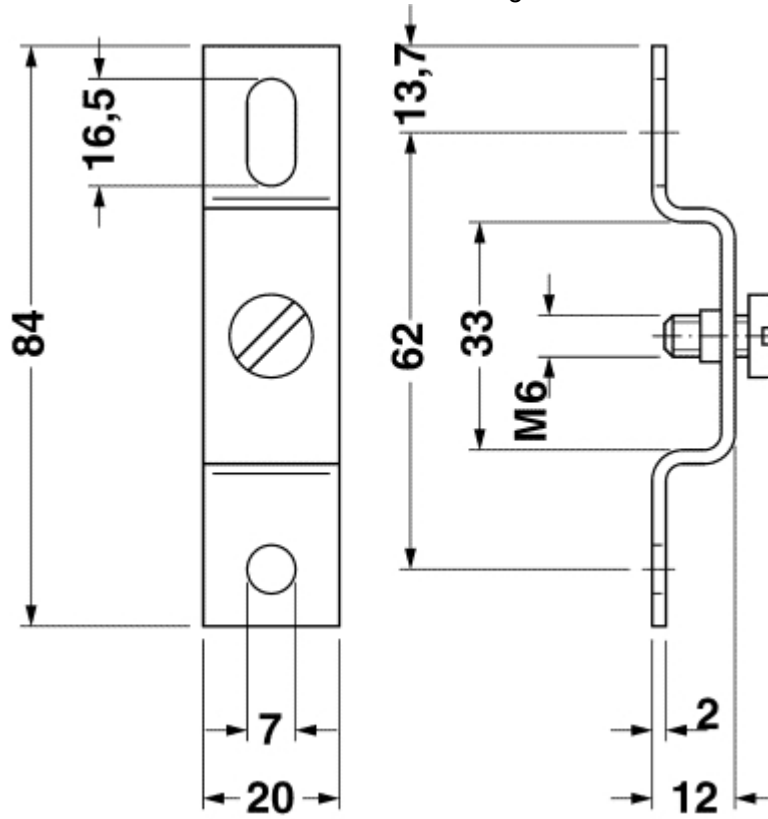
Dimensional drawing
