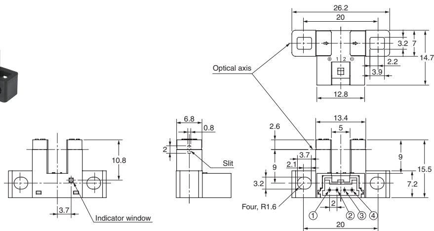
Mounting screw holes
