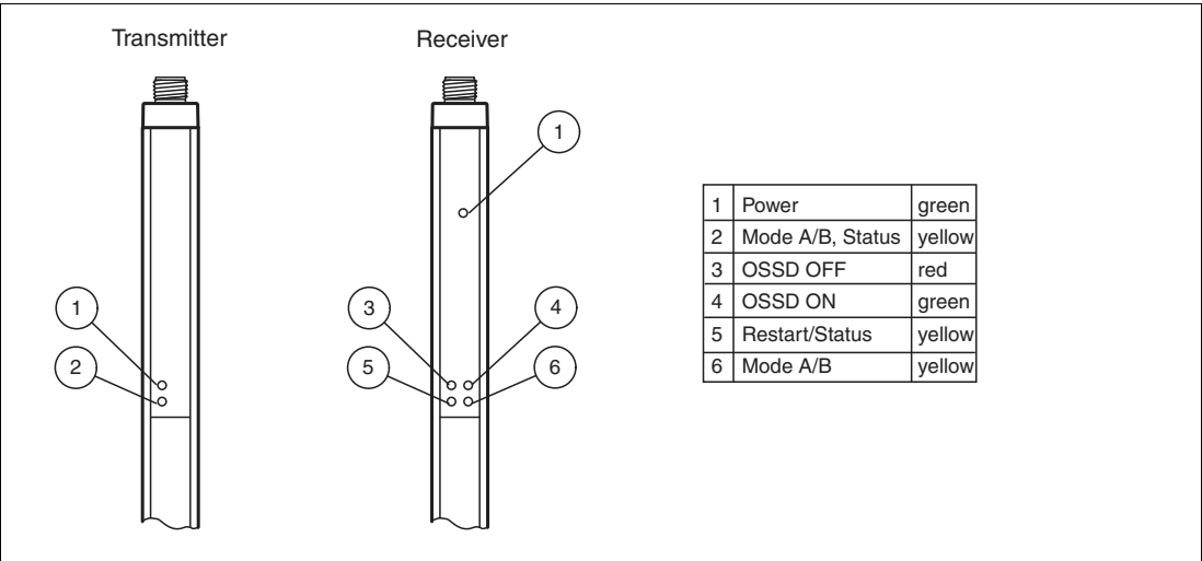
Figure 3.2 Displays on the transmitter and receiver units
