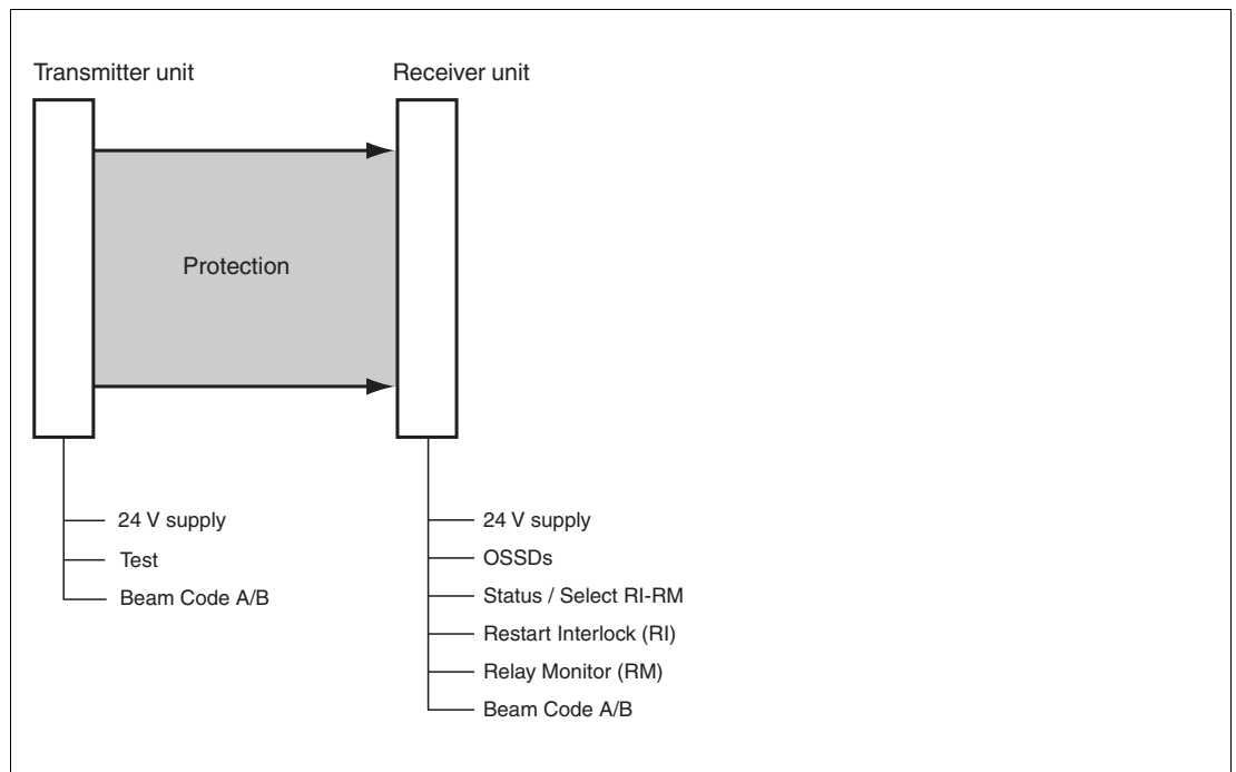
Figure 3.1 Schematic diagram of a detection device
