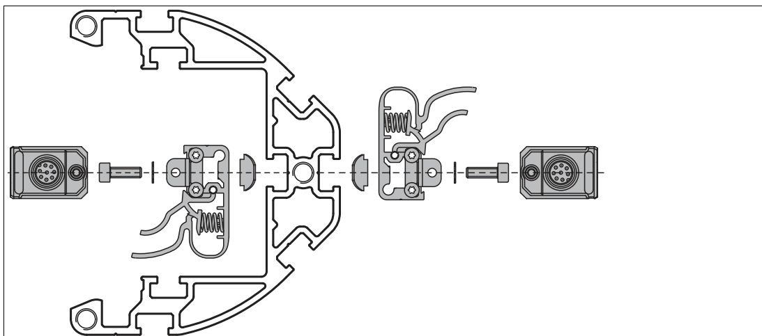
Figure 8.5 Example of mounting a mounting aid OMH-SLCT-01 to a mounting column
