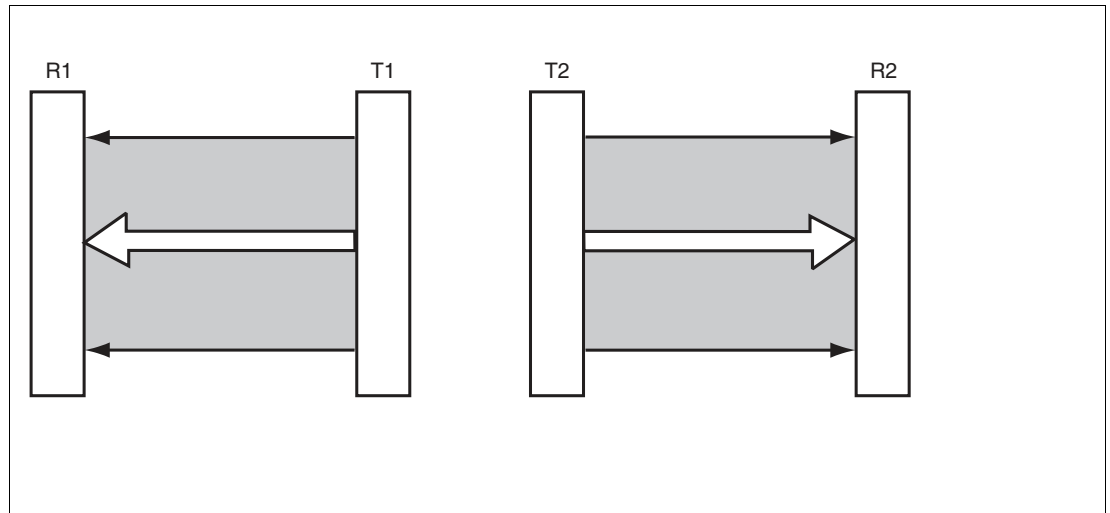
Figure 5.1 Multiple assignment
