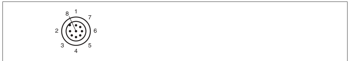
Figure 3.4 Pin assignment receiver unit
