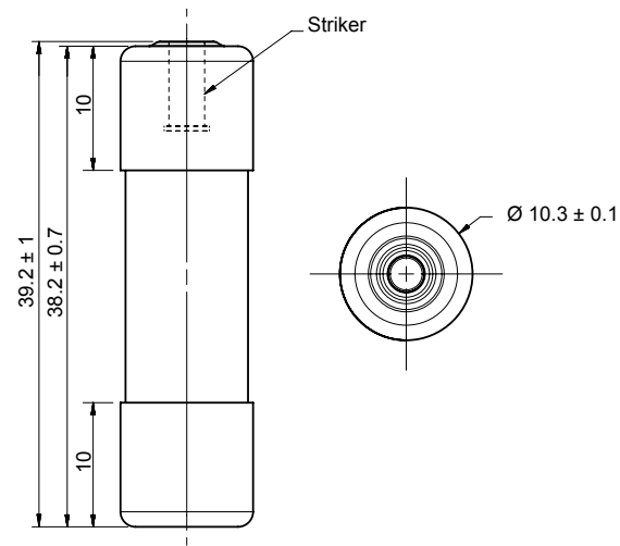
Size 10x38 aM with striker (33907)
