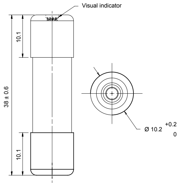
Size 10x38 aM with indicator (1002537)
