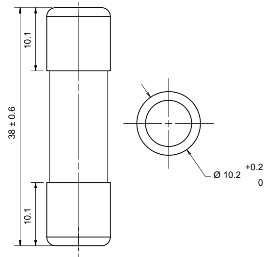
Size 10x38 aM without indicator (1001210)
