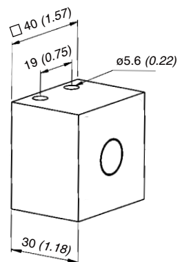
Standard Straight
