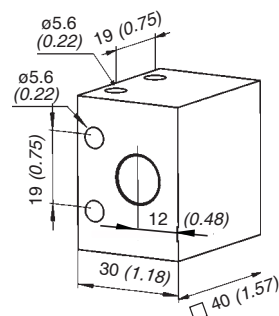
90° Side Entry
