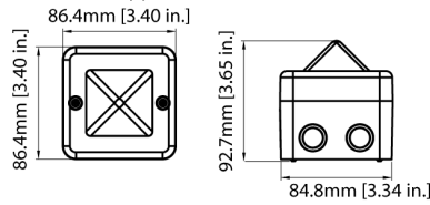
A100 Backbox (A)
