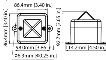
Multi-purpose Backbox (& IS-L101) (M)
