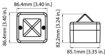
Multi-purpose Backbox (& IS-L101) (M)
