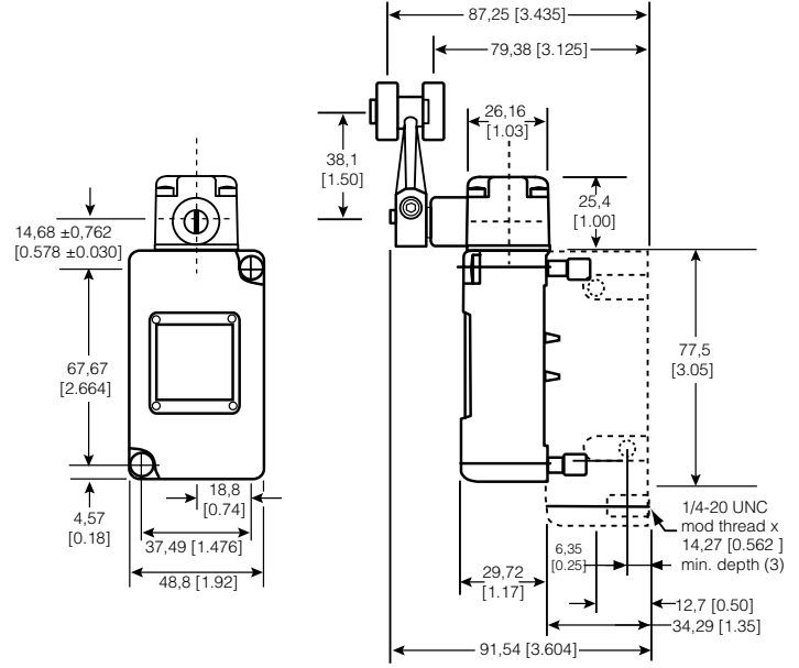
Figure 13. 201LS3 Dimensions
