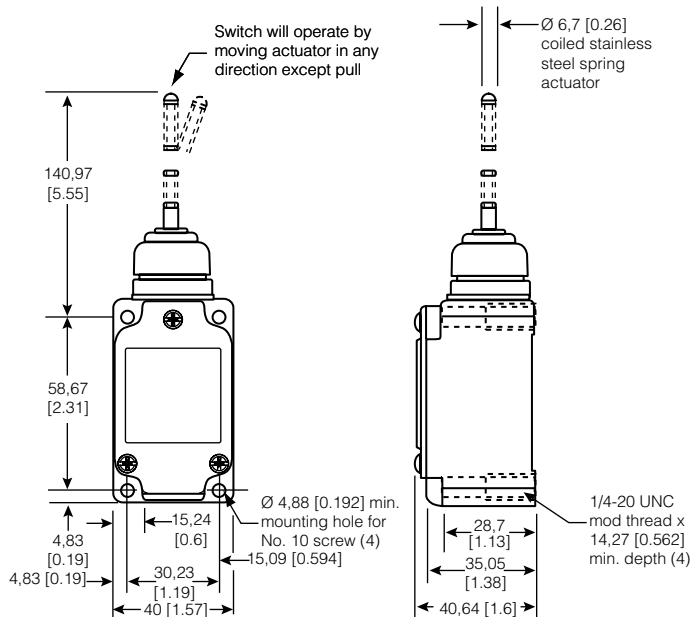
Figure 11. 8LS152 Dimensions
