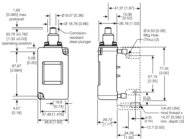
Figure 16. 203LS1 Dimensions
