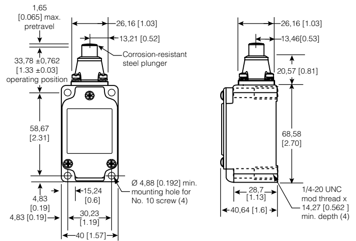
Figure 5. 3LS1 Dimensions
